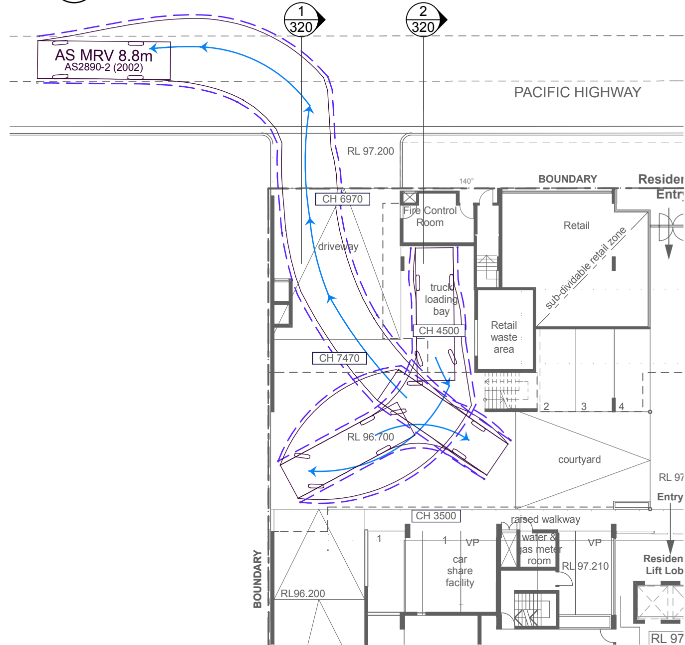
8.8 MRV Truck Out Plan
