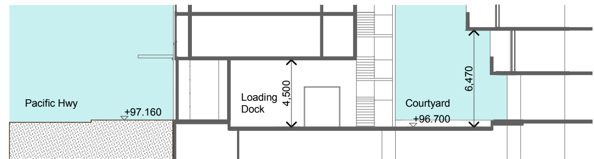
Section 2 Loading Dock
