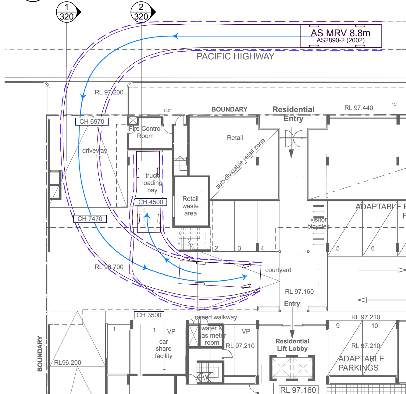
8.8 MRV Truck In Plan
